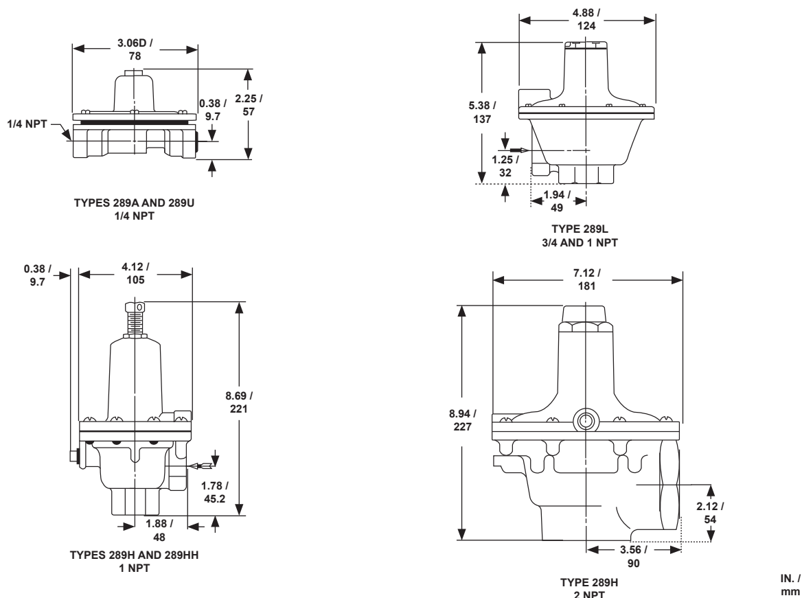
Figure 5. Dimensions
